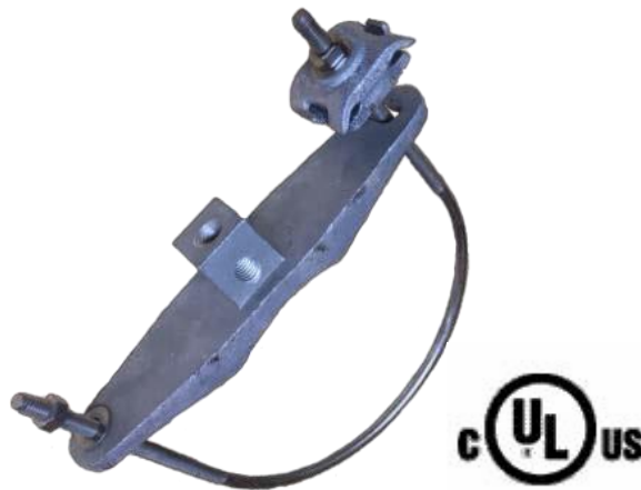
X6: Pipe Range 4.25" to 6.625"
